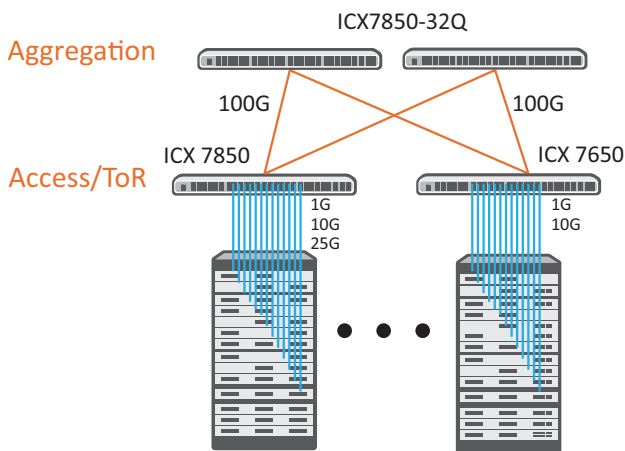
Figure 6: Data-Center Top of the Rack Connectivity.
